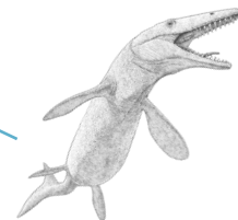
Mosasaur
